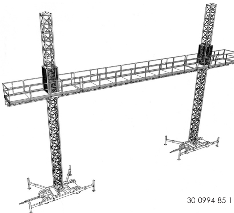
Drawing 1.4. SC1300 twin on wheel chassis.
