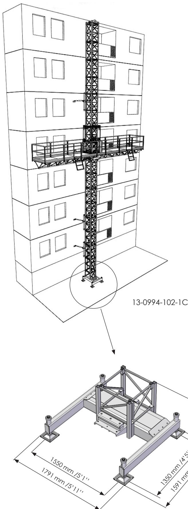
Drawing 1.7. SC1300 single on minichassis. Minichassis with dimensions.
